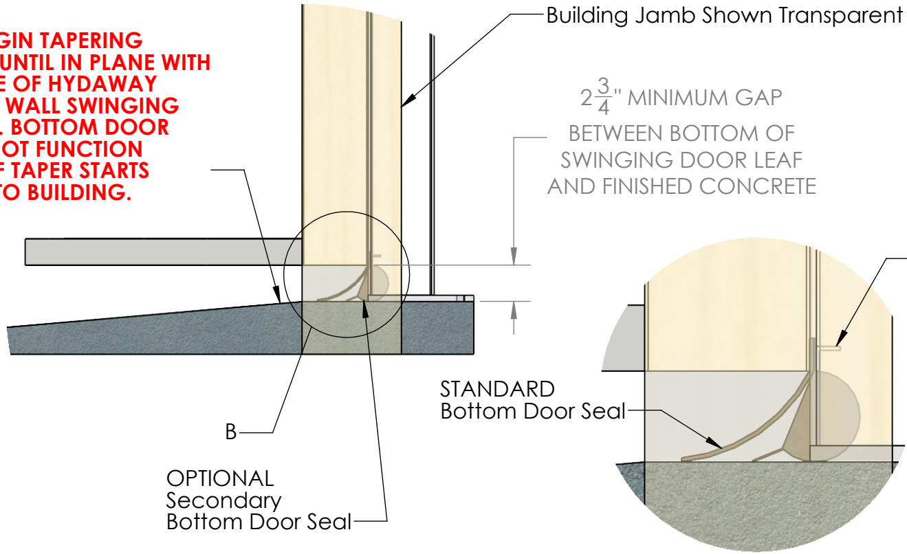
DETAIL B SCALE 1 : 4
