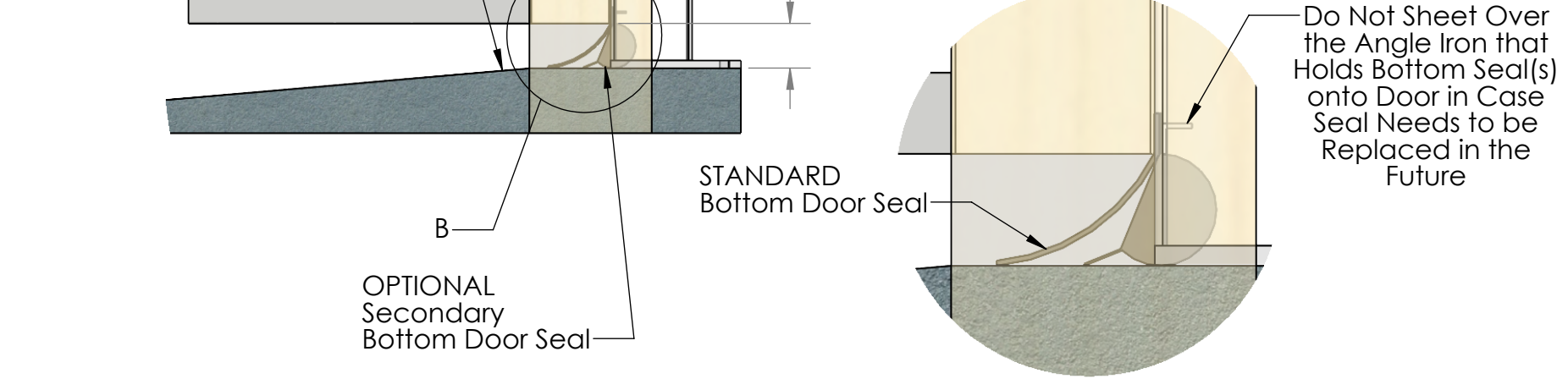
DETAIL B SCALE 1 : 4
